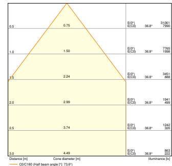
HB P 75W 840 110DEG IP66 PS - REFRACTOR
