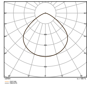
HB P 75W 840 110DEG IP66 PS
