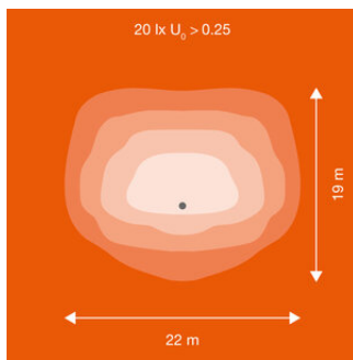
Streetlight Flex 80W RW35ST simplified isolux diagram
