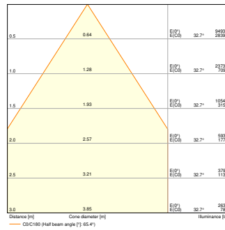
HB P 150W 865 70DEG IP66 PS
