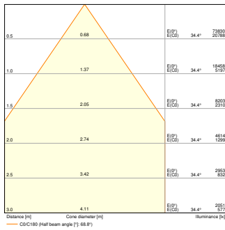
HB P 125W 865 70DEG IP66 PS
