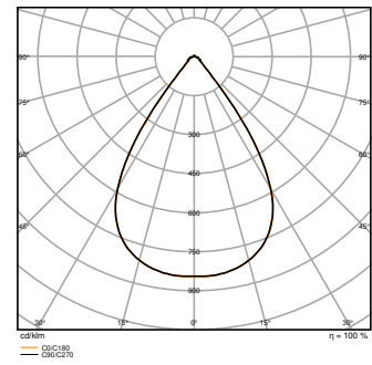
HB P 125W 865 70DEG IP66 PS
