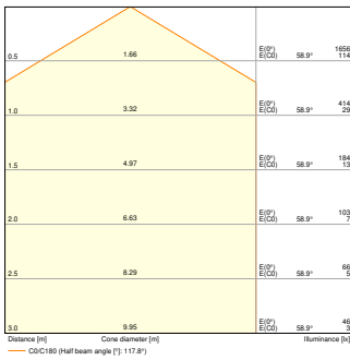
SF CIRC 500 V 42W 830 IP44 PS 1500lm
