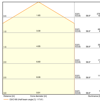
SF CIRC 500 V 42W 830 IP44 PS 2500lm
