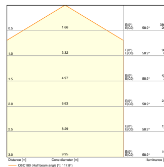
SF CIRC 500 V 42W 830 IP44 PS 3500lm
