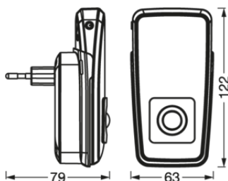
PGLUNETTA TORCH INDUCTIVE SENSOR WTMiPRCmkn
