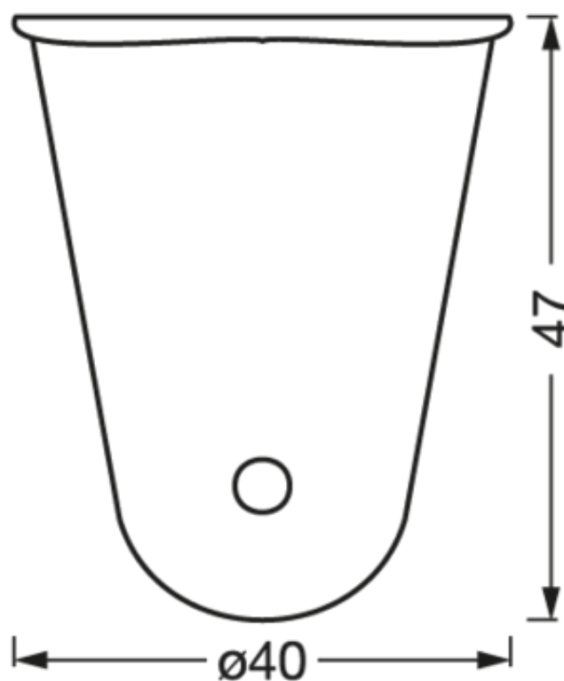
TRACKLIGHT SUSPENSION KIT WT
