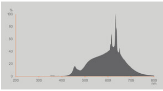
Spectral graph classic B 2700K DIM
