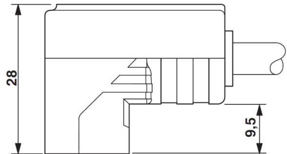
valve plug, design C
