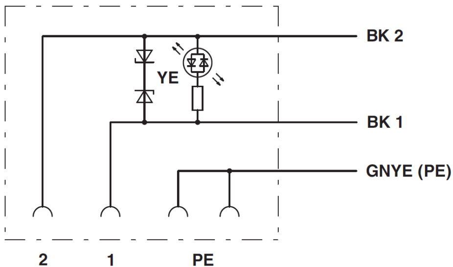
Contact the valve plug
