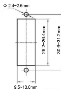
Mounting cutout
